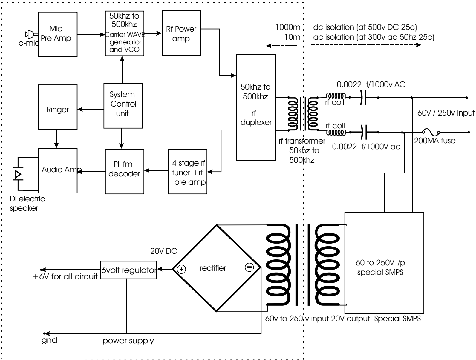
(New) schematic diagram of thodukonics powerfone power line wireless intercom model mci06b visit : www.thodukonics.com
